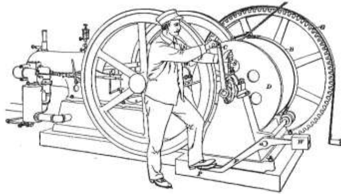
Figure E 5.23. This type of gasoline hoist was employed at vertical and inclined shafts from the 1900s to the 1930s. A single-cylinder engine is at left, dual flywheels are at center, and the cable drum is at right. Source: International Textbook Company, 1906, A50:31.
