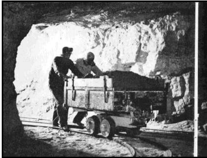
Figure E 5.11: Ore cars were the most popular means used to haul rock out of productive mines during the uranium industry's history. They carried between one and two tons of material. Mesa Miracle, 1951:6.
