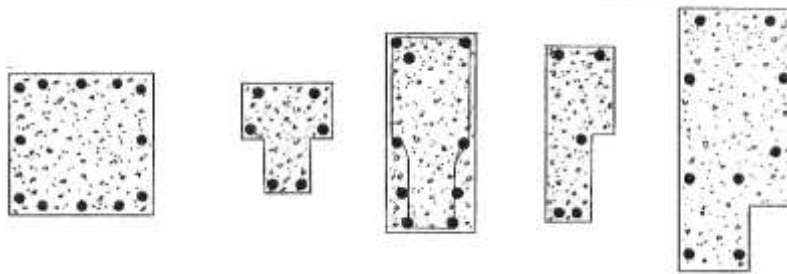
Figure E 5.24. Hoist foundation plan views. Single-drum steam hoists were bolted to foundations like the one at left, and the other foundations were for various types of gasoline hoists. Source: Twitty, 2002:187, 241.
