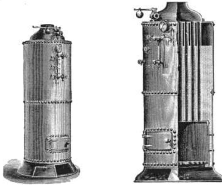
Figure E 5.19. Upright boilers were the least expensive and most portable type of boiler, but they were also inefficient. Flue gases rose from the firebox at bottom, through the flue tubes, and out a smokestack at top. Note the water level sight tube, pressure gauge, and pressure valve. Source: Rand Drill Company, 1886:47.
