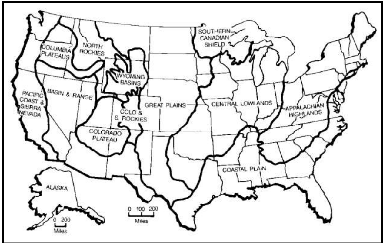
Figure E 3.1: The map illustrates North America's principal geological regions. The Colorado Plateau radiates outward from the Four Corners area, at lower right. Colorado, and in particular Montrose and San Miguel counties, featured most of the ore bodies on the Plateau. Source: U.S. Uranium Mining, 1984:22.
