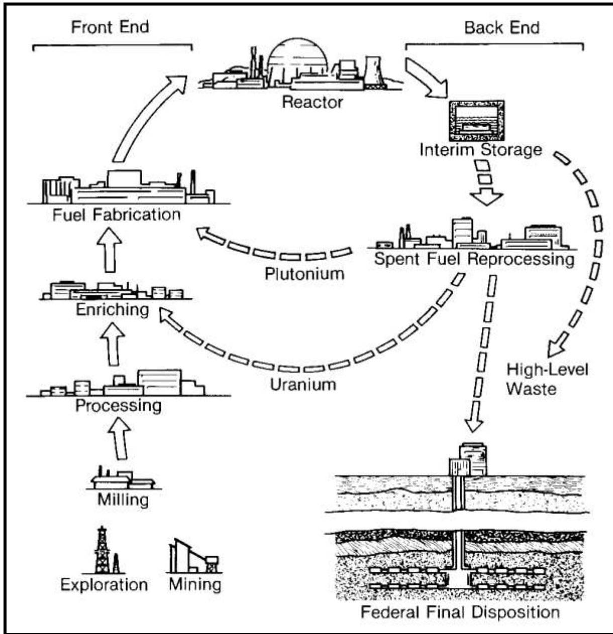
Figure E 4.15: The diagram neatly illustrates the lifecycle of uranium fuel for the nuclear power industry. Western Montrose and San Miguel counties were important centers of exploration, mining, and milling. The Atomic Energy Commission oversaw all steps. Source: U.S. Uranium Mining, 1984:73.
