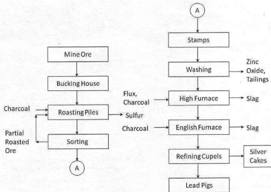
Silver Hill Mine flowsheet, 1852.
