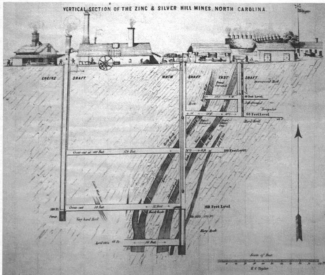
Zinc and Silver Hill Mines (Silver Hill Mine) cross-section, 1854. (From Schoonmaker, Statement of the Condition and Prospects.)
