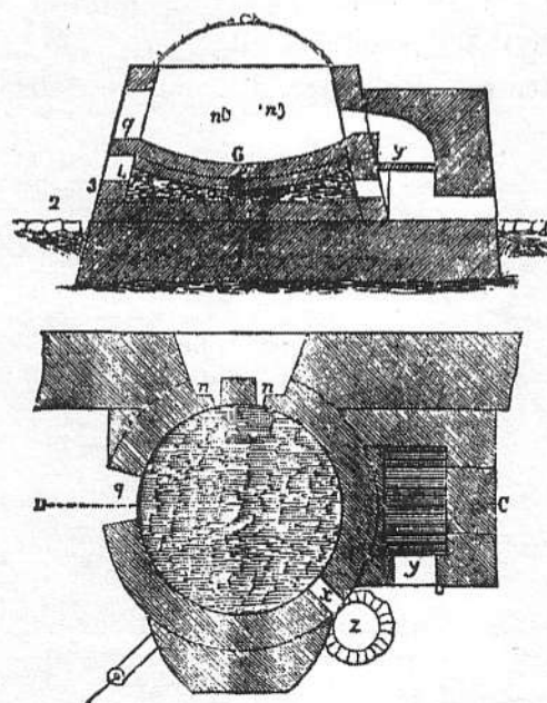
German refining furnace (From Tenney, "Gold and Silver Produced in the Mines of America.")
