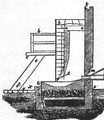
High furnace (From Tenney, "Gold and Silver Produced in the Mines of America.")
