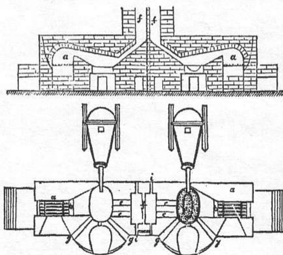
English reverberatory refining furnace. (From Tenney, "Gold and Silver Produced in the Mines of America.")
