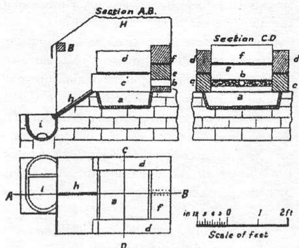
Scotch hearth furnace. (From Collins, Metallurgy of Lead.)
